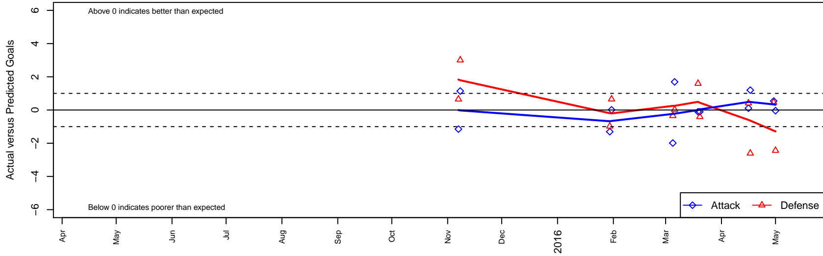
Utah Avalanche ECNLG00 Dots are actual minus expected GF (blue circles) and GA (red triangles). Blue line is smoothed change in attack strength. Red is smoothed change in defense strength.
